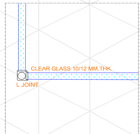
DETAIL OF 'L' JOINT PROFILE
