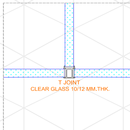
DETAIL OF 'T' JOINT PROFILE
