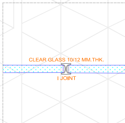
DETAIL OF 'I' JOINT PROFILE
