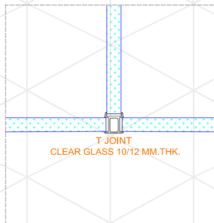
DETAIL OF 'T' JOINT PROFILE
