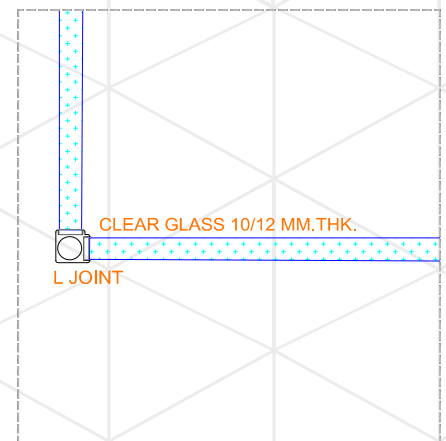
DETAIL OF 'L' JOINT PROFILE
